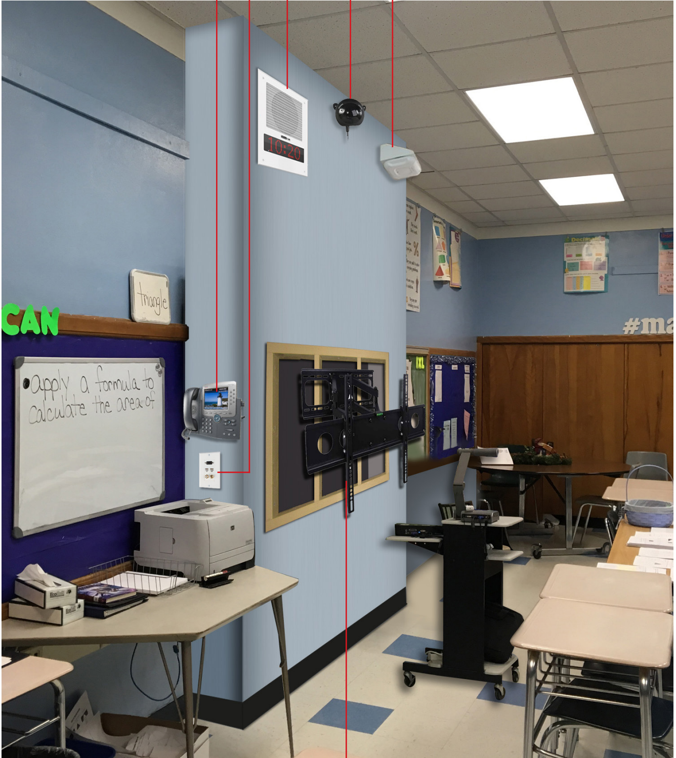
Wall opening with flat-screen TV mounting bracket
